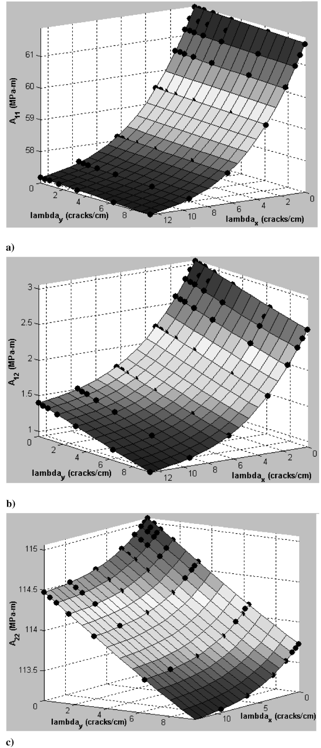
Fig. 6 Complete cubic polynomial fit using least squares approximation over 56 data points (black dots) obtained from FE simulations. a) A_{11} , b) A_{12} , and c) A_{22} .
